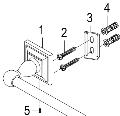
24" Towel Bar
