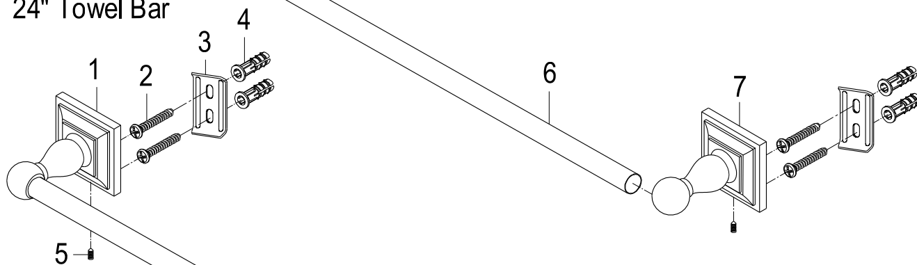
24" Towel Bar
